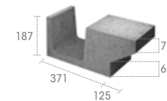
RS 905 Escalera cerrada Closed built-in stairs Échelle fermée
