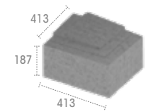
RS 918 Esquina exterior Outside corner Angle extérieur
